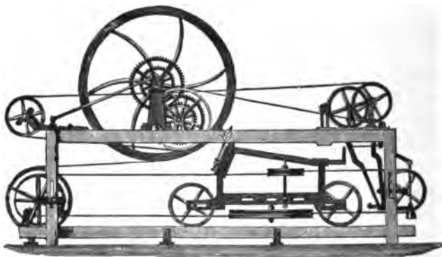
CROMPTON'S MULE-JENNY (specification drawing).
